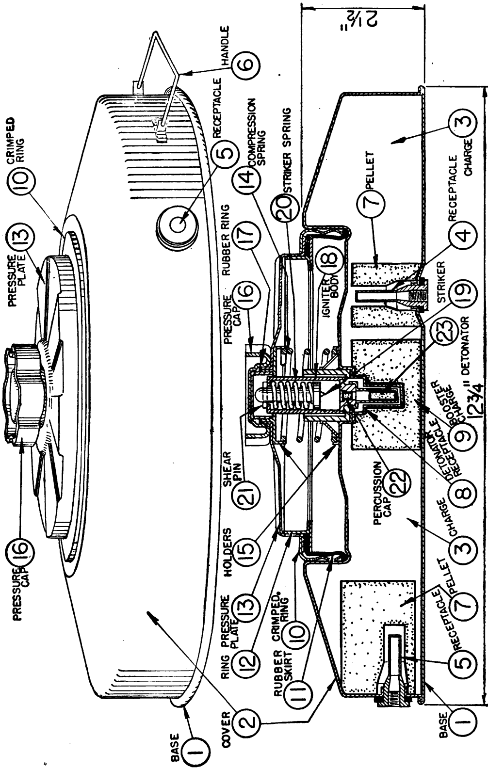
FIGURE 24.1.—Tellermine No. 2.
